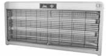
Fly Catcher Size: 610x60x270mm, 40W Size: 505x60x270mm, 30W Size: 395x60x270mm, 20W
